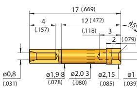
KT-254 L3 E02 - 30 (Solder Connection)
