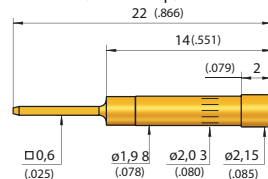
KT-254 W-PL (wire-wrap)
