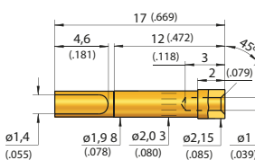
KT-254 L3 E02 - 30 (Solder Connection)
