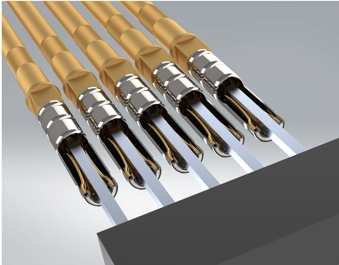
Cut view of contacting
